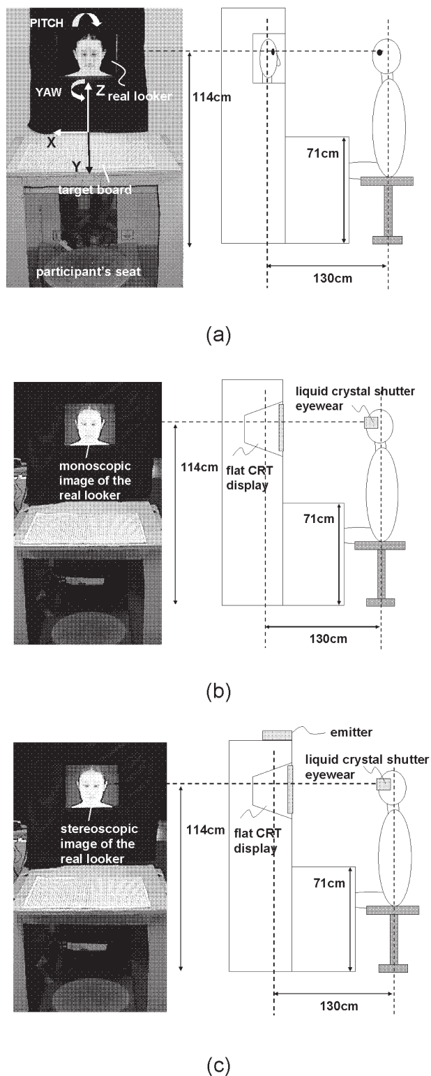
Figure 1. Experimental environments. (a) Face-to-face experiment. (b) Monoscopic image experiment. (c) Stereoscopic image experiment. The image was presented by a time-multiplexed stereoscopic CRT display with refresh rate 120 Hz.
